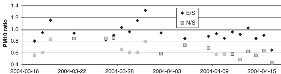
Fig. 5. Ratio of the daily average PM10 levels at the washed stretch (E) and the CMA treated stretch (N) compared to the untreated stretch (S) in spring 2004 at Vallstanäs.
