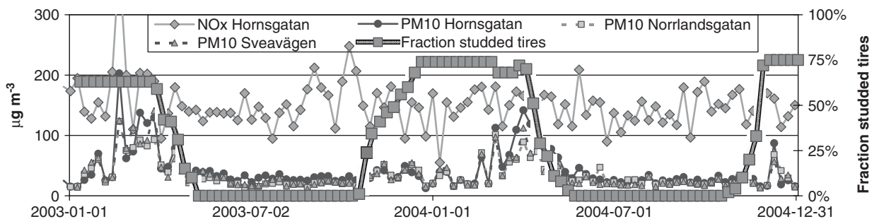
Fig. 1. Weekly average PM 10 and NO x levels together with the fraction of studded tyres on light duty vehicles in Stockholm City.
