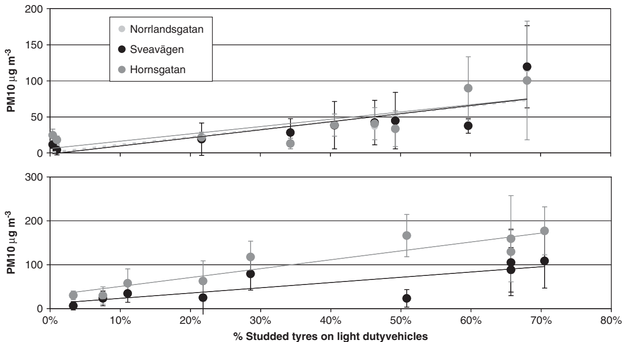
Fig. 3. Scatter plot of weekly average PM10 levels in Stockholm City against fraction of studded winter tyres on light duty vehicles. Upper panel: data from October–December 2003. Lower panel: data from February–May 2004. Only data during dry street conditions daytime has been included. The vertical bars denote the standard deviation.
