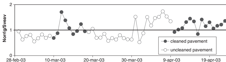
Fig. 4. Daily average PM10 ratios between Norrlandsgatan and Sveavägen during March and April 2003.
