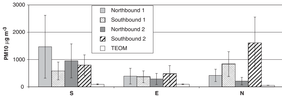
Fig. 6. The average PM10 concentrations along the highway 20 m behind a car that is driving in the verge of the highway. The driving speed for northbound 1 and 2 were 70 and 90 km h -1 , respectively, and the same for southbound 1 and 2. The vertical bars represent the standard deviation. “S” denotes the untreated stretch, “E” the washed stretch and “N” the CMA treated stretch.
